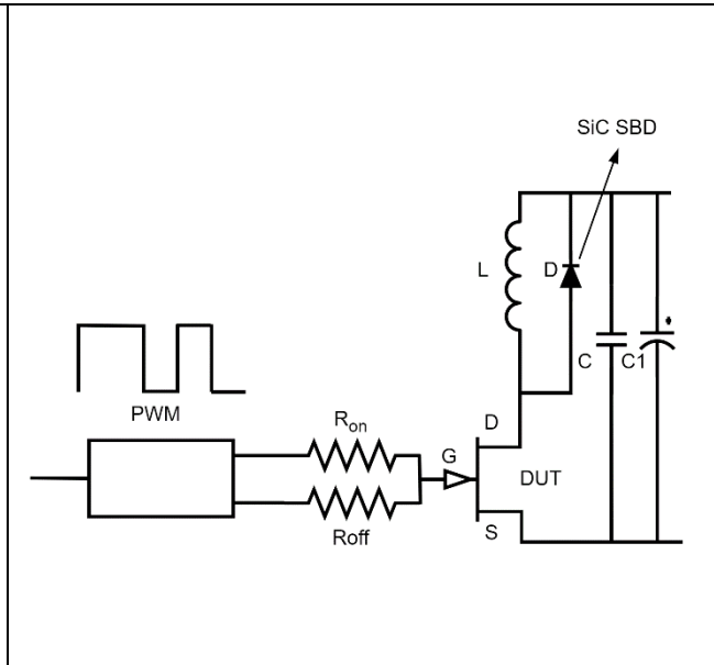
Figure 14: DPT circuit used for switching times measurement, V_{DS} = 400\text{ V} , I_{DS} = 6\text{ A} , L = 400\text{ }\mu\text{H} , V_{GS} = 6\text{ V} , R_{on} = 10\text{ }\Omega , R_{off} = 2.2\text{ }\Omega
