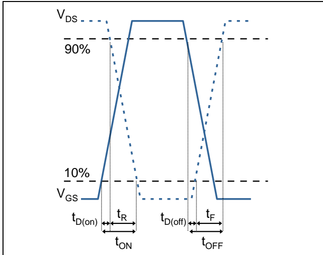
Figure 15: Typical Switching times waveform
