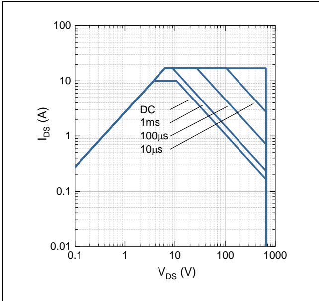
Figure 13: Safe Operating Area at T_{case} = 25\text{ }^{\circ}\text{C}
